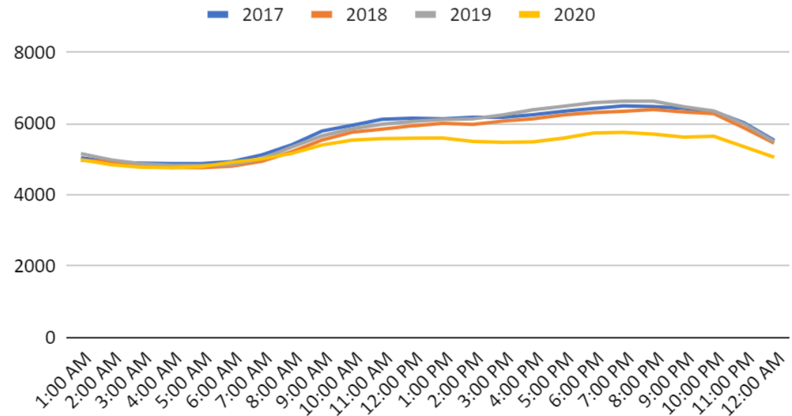
Sunday Usage (MWh)
