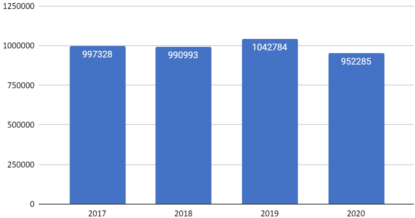
Bonneville Power Administration Weekly Electricity Demand (MWh) June 12 - June 18
